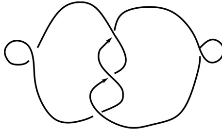
FIGURE 50. T_{2,-3} .
