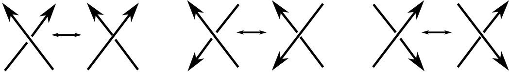
FIGURE 27. Transverse crossing changes.
