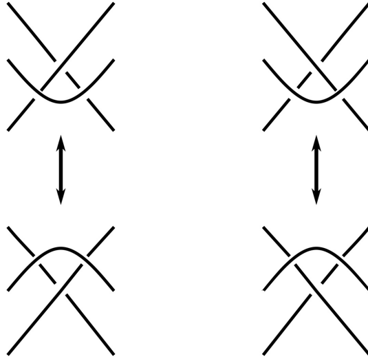
FIGURE 25. Transverse Type III Reidemeister moves.
