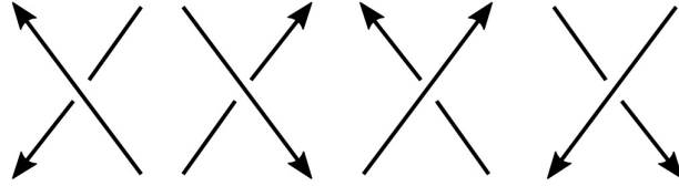
FIGURE 16. Positive crossings.
