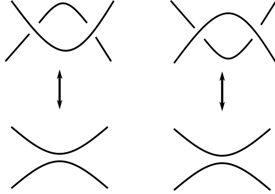
FIGURE 24. Transverse Type II Reidemeister moves.
