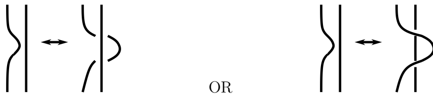
FIGURE 7. Type II Reidemeister moves.
